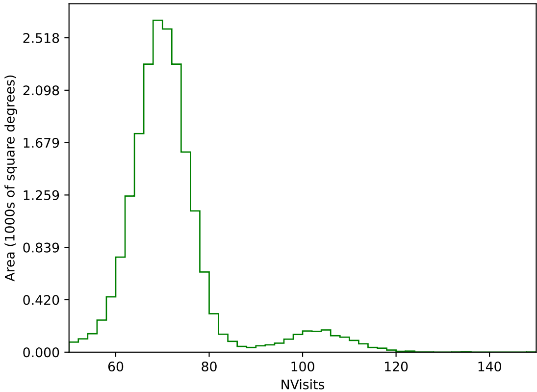
ddf_acor_sf10_lsf20_lsr20_v3.4_10yrs All sky g band: NVisits
