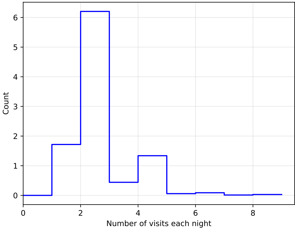
ddf_acor_sf10_lsf20_lsr20_v3.4_10yrs All sky: NVisitsPerNight 1e6
