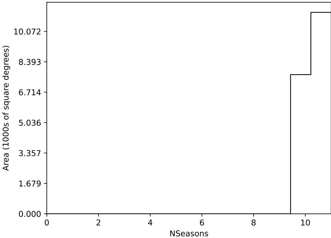
ddf_acor_sf10_lsf20_lsr20_v3.4_10yrs WFD all bands: NSeasons
