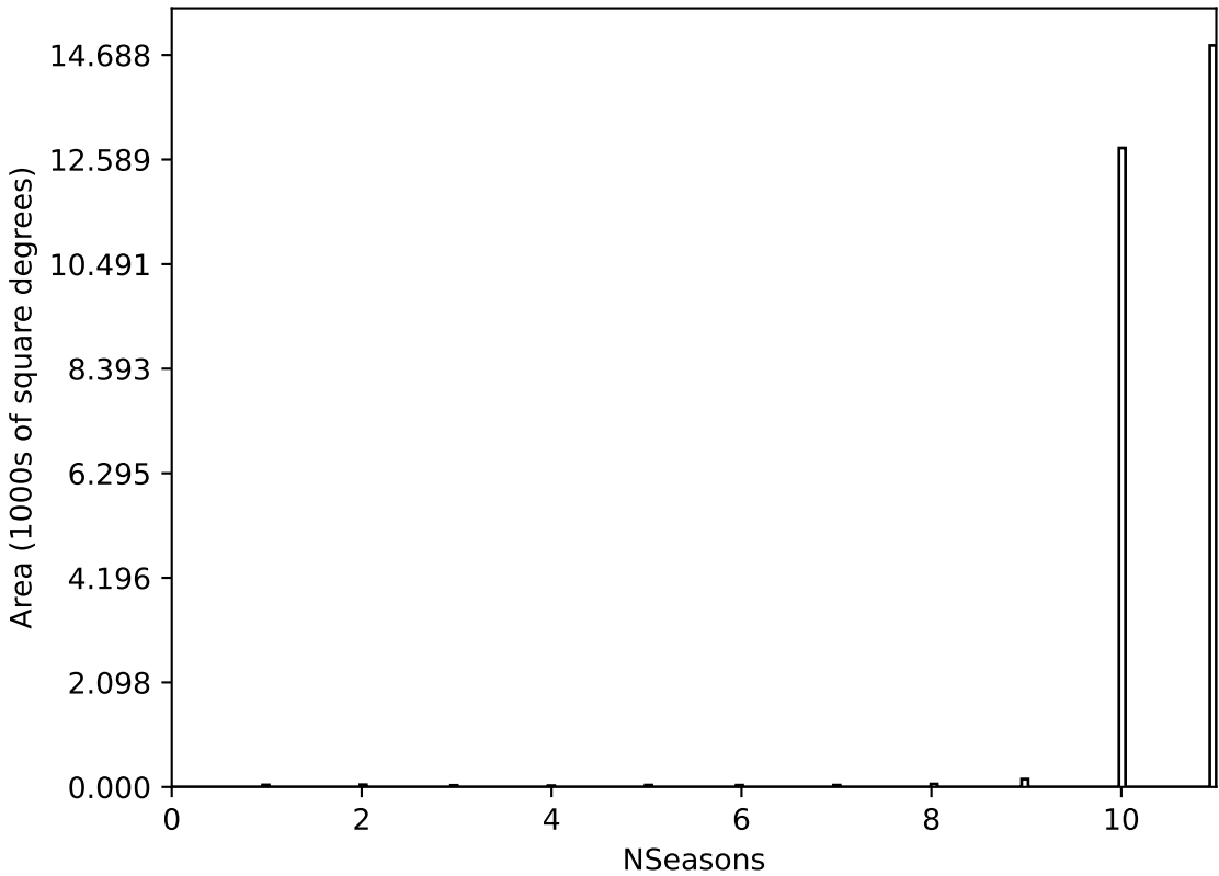
ddf_acor_sf10_lsf20_lsr20_v3.4_10yrs All sky all bands: NSeasons
