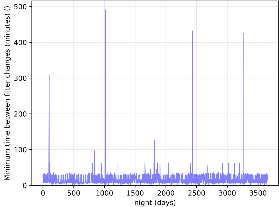
ddf_acor_sf10_Isf20_Isr20_v3.4_10yrs Per Night: Minimum time between filter changes (minutes)
