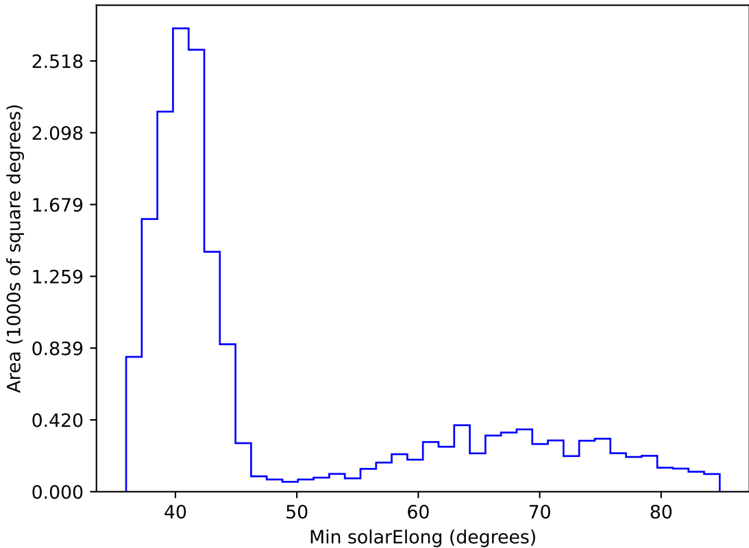
ddf_acor_sf10_lsf20_lsr20_v3.4_10yrs WFD z band: Min solarElong
