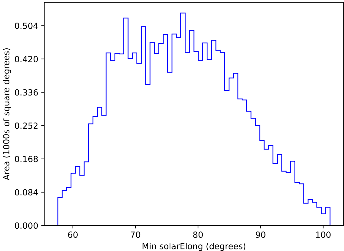
ddf_acor_sf10_lsf20_lsr20_v3.4_10yrs WFD u band: Min solarElong
