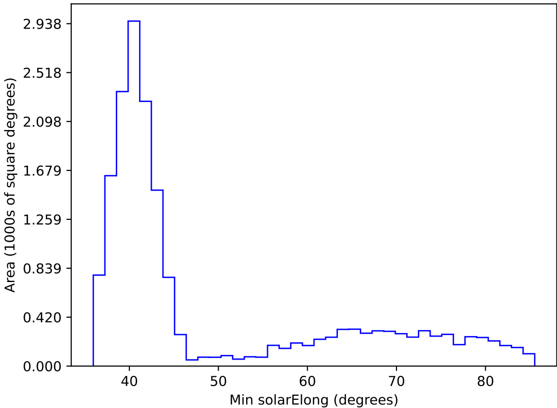
ddf_acor_sf10_lsf20_lsr20_v3.4_10yrs WFD i band: Min solarElong
