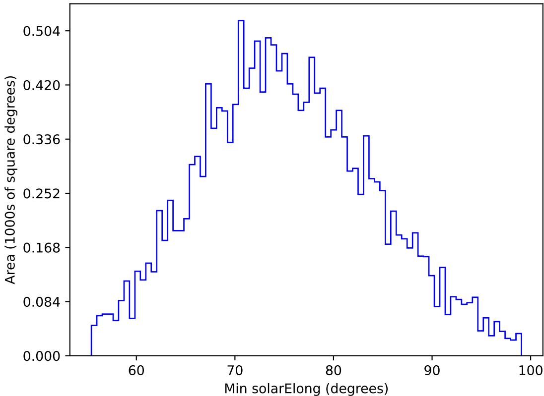
ddf_acor_sf10_lsf20_lsr20_v3.4_10yrs WFD g band: Min solarElong
