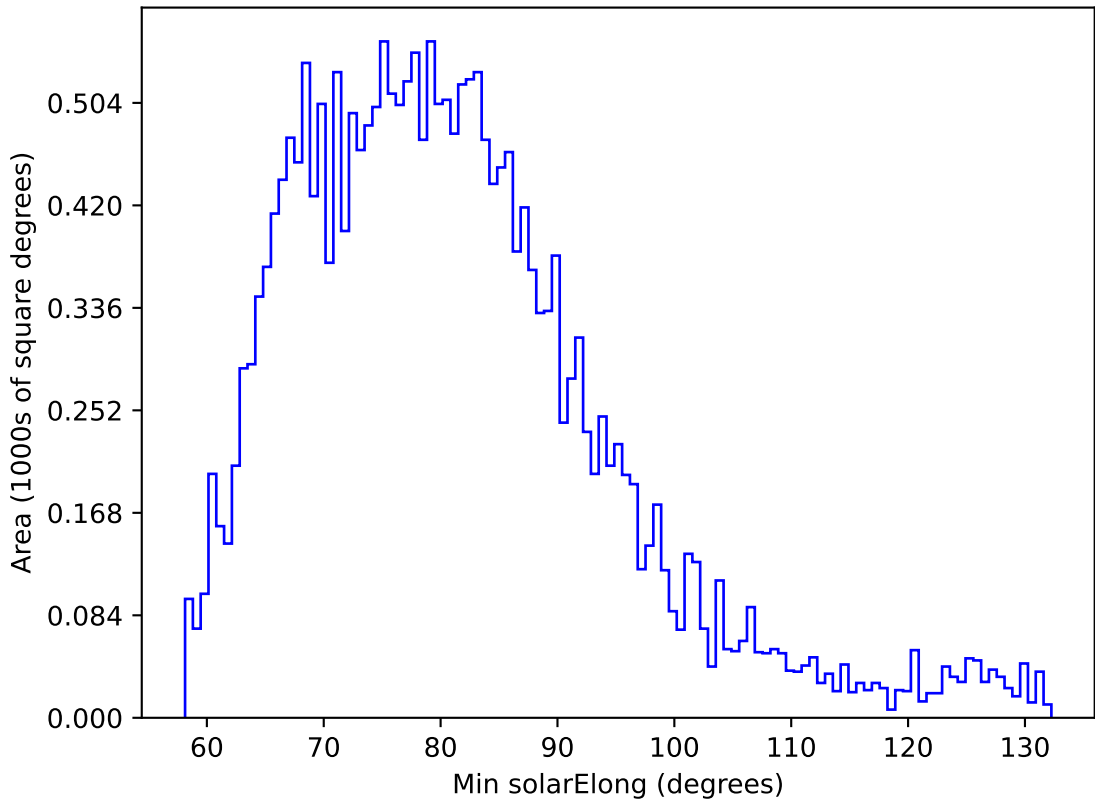
ddf_acor_sf10_lsf20_lsr20_v3.4_10yrs All sky u band: Min solarElong
