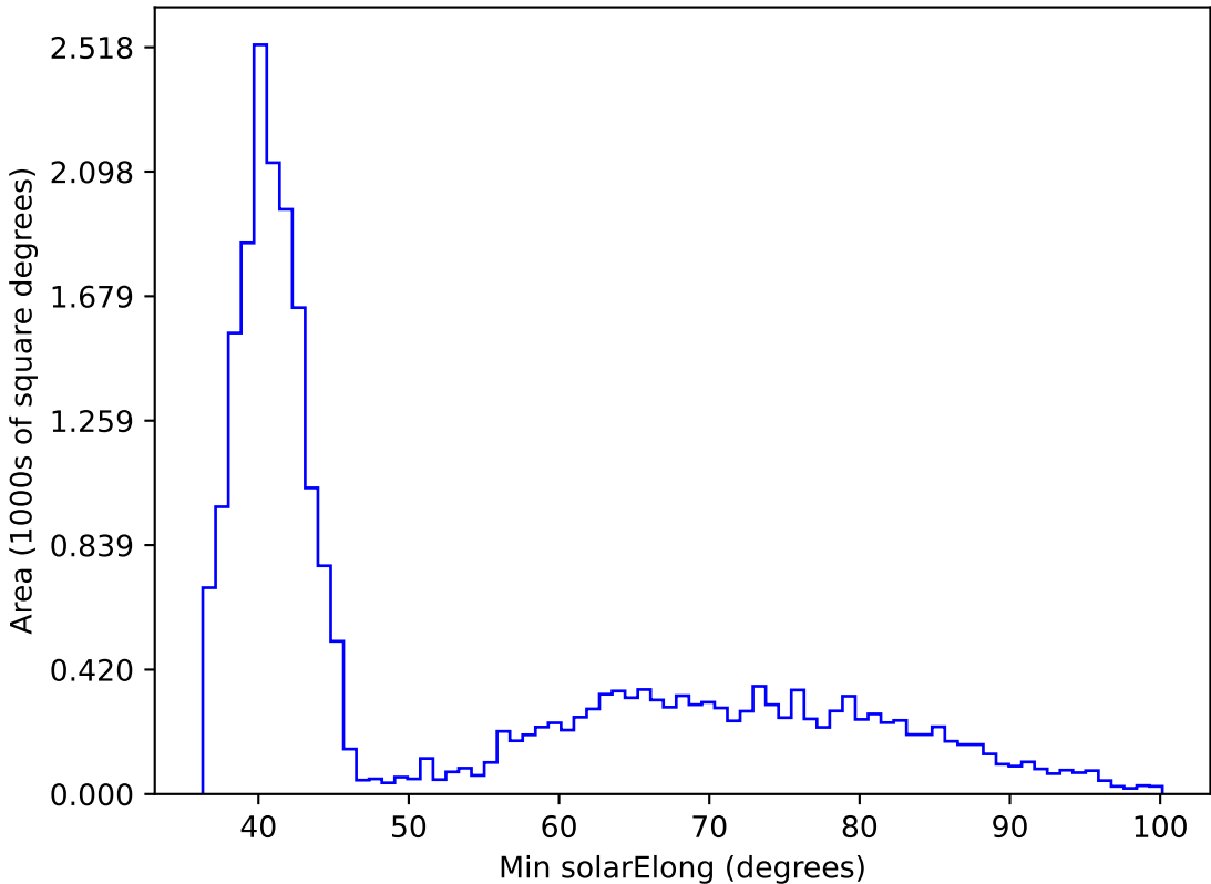
ddf_acor_sf10_lsf20_lsr20_v3.4_10yrs All sky i band: Min solarElong
