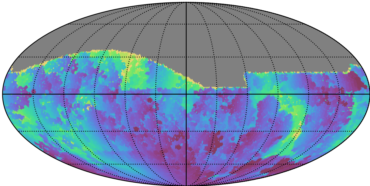
ddf_acor_sf10_lsf20_lsr20_v3.4_10yrs All sky g band: Min solarElong
