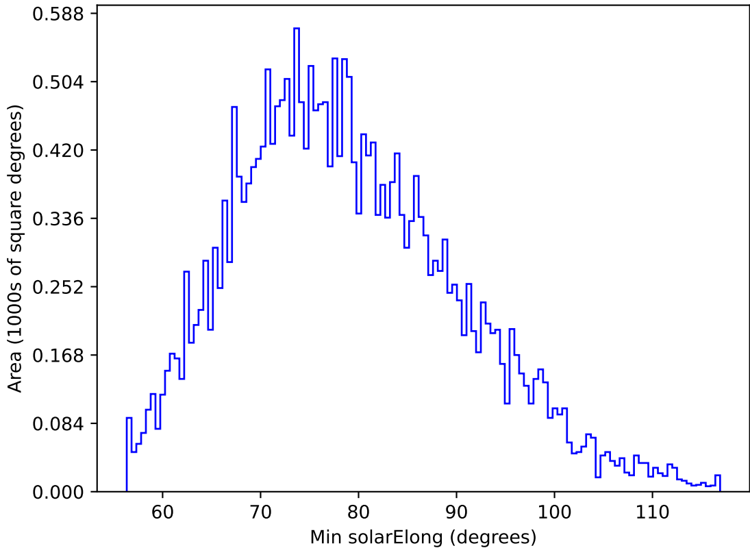
ddf_acor_sf10_lsf20_lsr20_v3.4_10yrs All sky g band: Min solarElong
