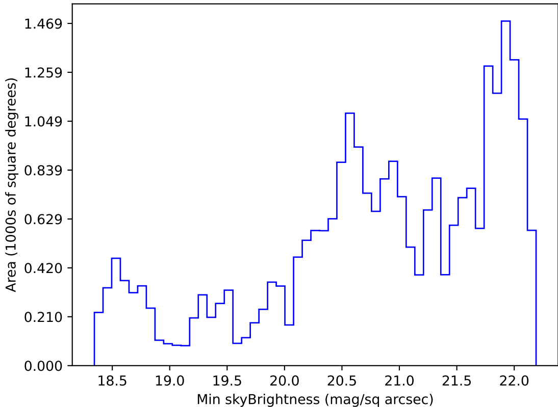
ddf_acor_sf10_lsf20_lsr20_v3.4_10yrs Yr 1 g band: Min skyBrightness
