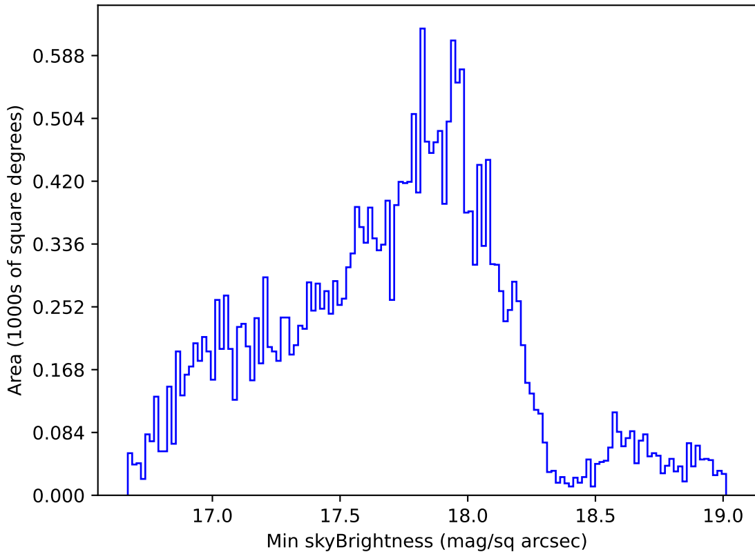
ddf_acor_sf10_lsf20_lsr20_v3.4_10yrs Yr 1 all bands: Min skyBrightness
