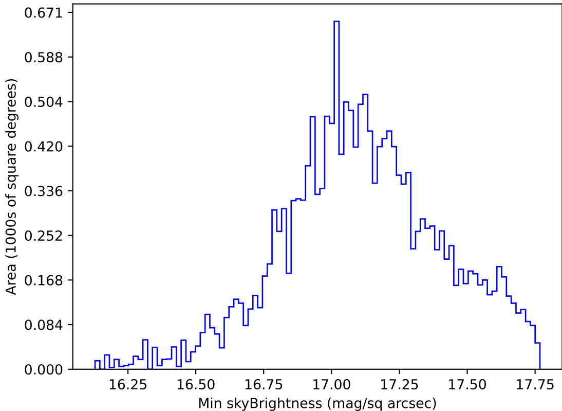
ddf_acor_sf10_lsf20_lsr20_v3.4_10yrs WFD y band: Min skyBrightness
