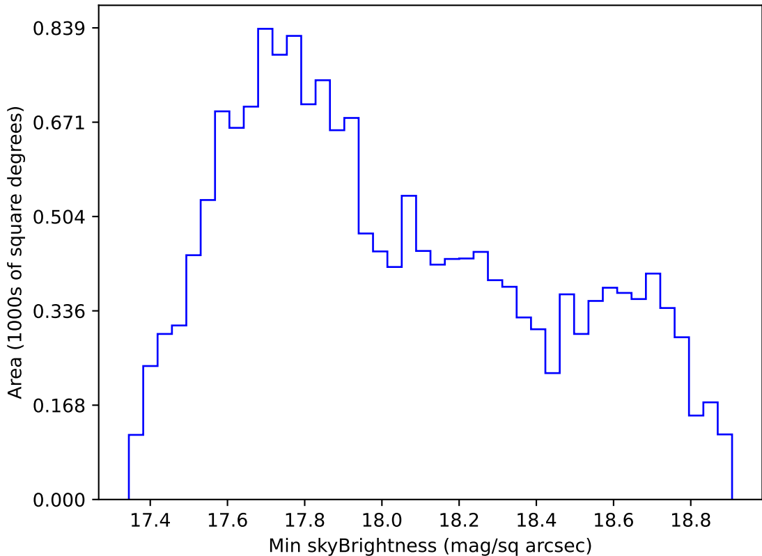
ddf_acor_sf10_lsf20_lsr20_v3.4_10yrs WFD i band: Min skyBrightness
