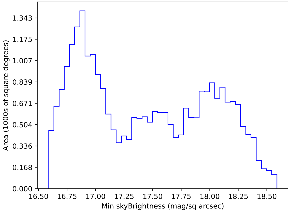
ddf_acor_sf10_lsf20_lsr20_v3.4_10yrs All sky z band: Min skyBrightness
