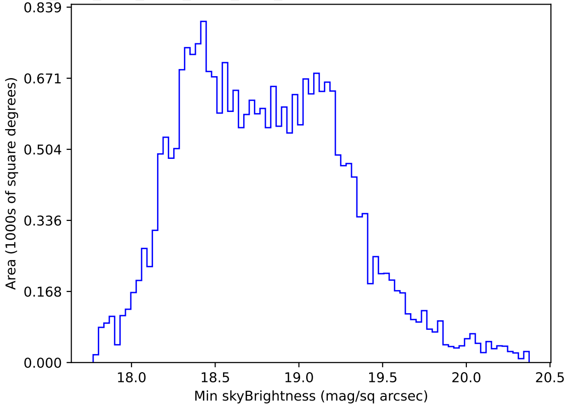
ddf_acor_sf10_lsf20_lsr20_v3.4_10yrs All sky r band: Min skyBrightness
