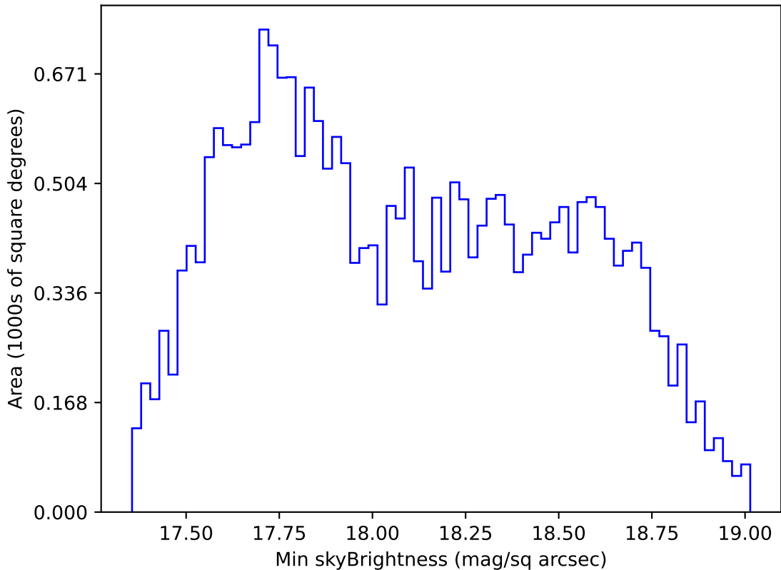
ddf_acor_sf10_lsf20_lsr20_v3.4_10yrs All sky i band: Min skyBrightness
