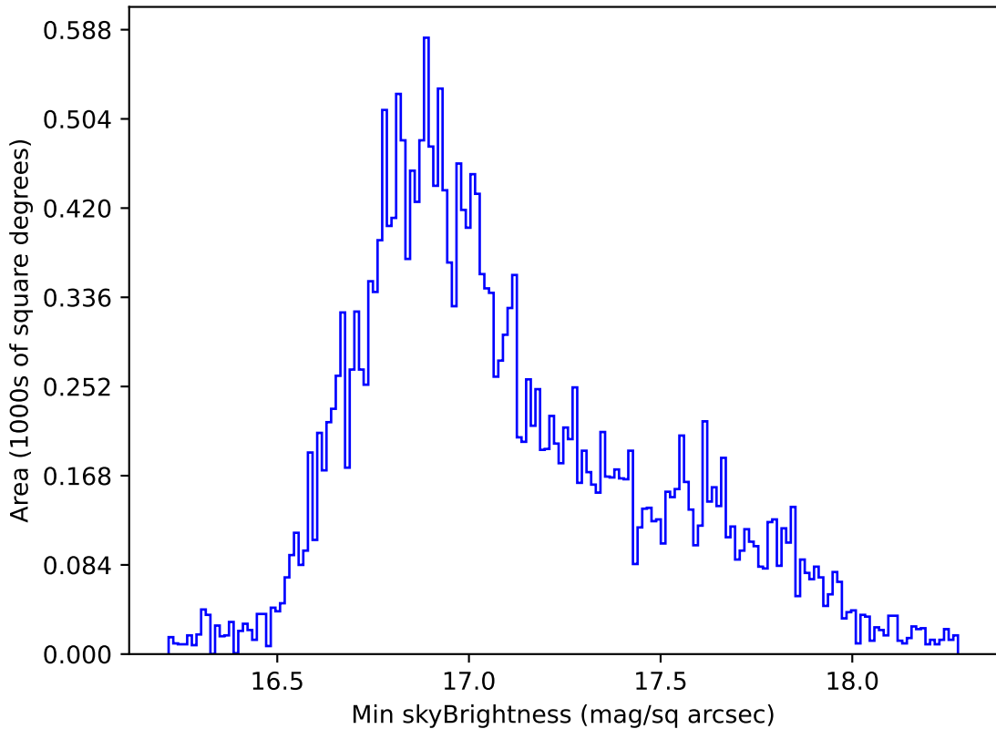
ddf_acor_sf10_lsf20_lsr20_v3.4_10yrs All sky all bands: Min skyBrightness
