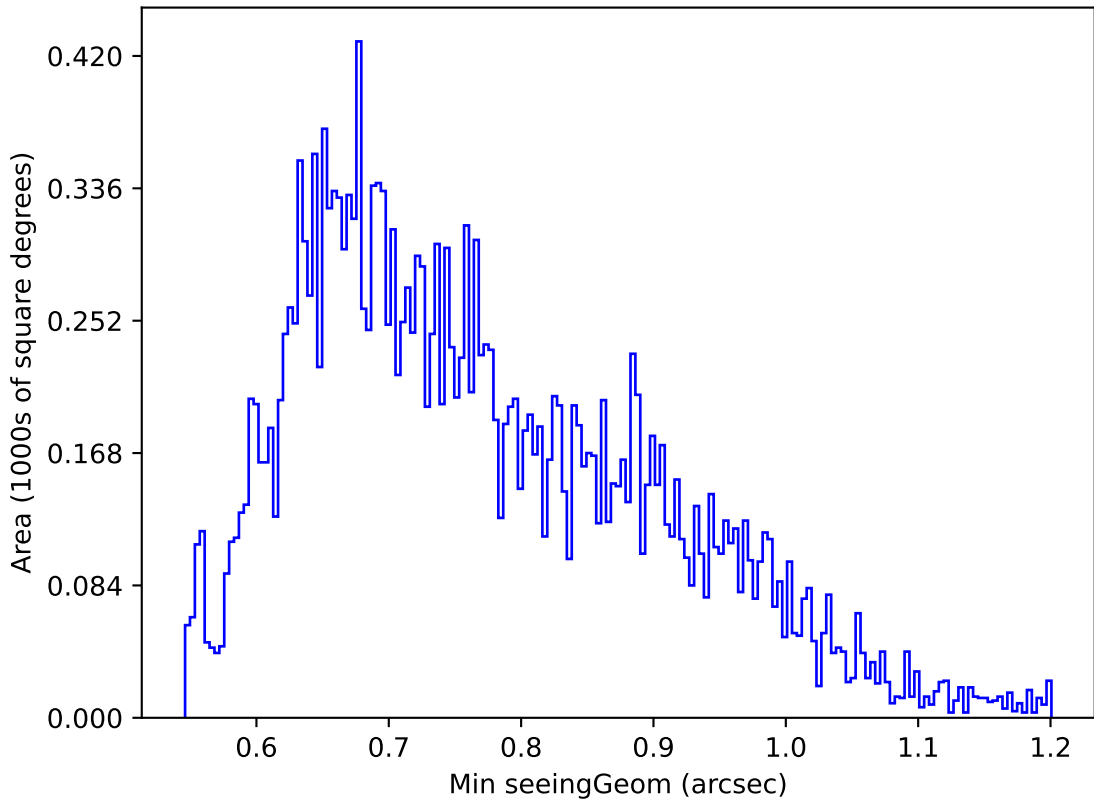
ddf_acor_sf10_ls20_lsr20_v3.4_10yrs Yr 1 u band: Min seeingGeom
