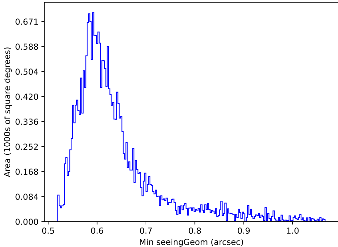
ddf_acor_sf10_lsf20_lsr20_v3.4_10yrs Yr 1 i band: Min seeingGeom
