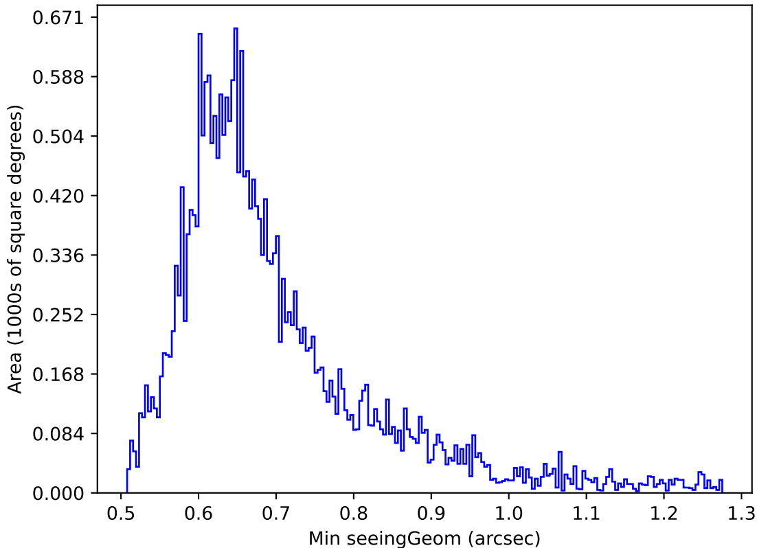
ddf_acor_sf10_ls20_lsr20_v3.4_10yrs Yr 1 g band: Min seeingGeom
