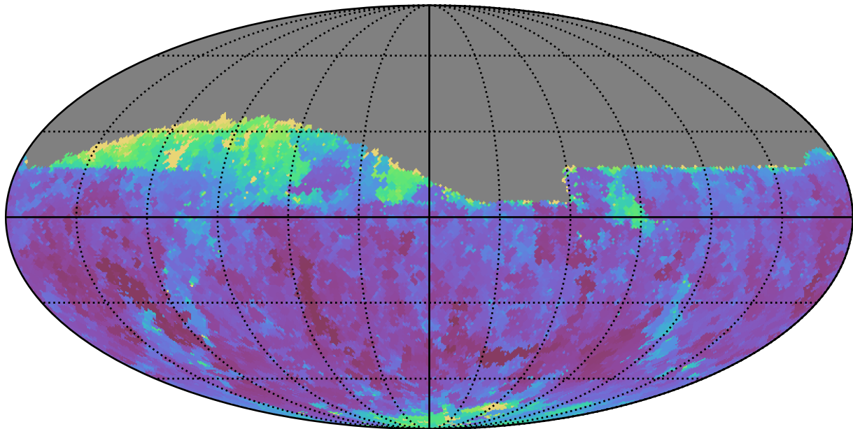
ddf_acor_sf10_lsf20_lsr20_v3.4_10yrs Yr 1 z band: Min seeingEff
