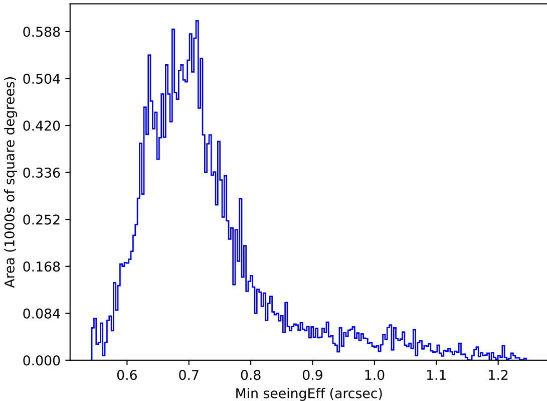
ddf_acor_sf10_ls20_lsr20_v3.4_10yrs Yr 1 z band: Min seeingEff
