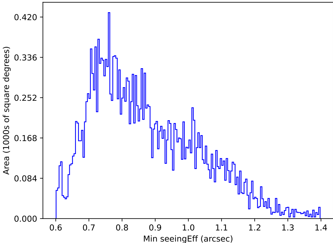
ddf_acor_sf10_lsf20_lsr20_v3.4_10yrs Yr 1 u band: Min seeingEff
