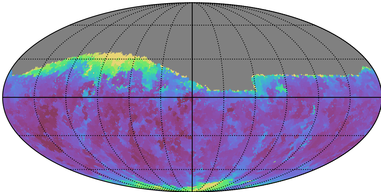
ddf_acor_sf10_lsf20_lsr20_v3.4_10yrs Yr 1 r band: Min seeingEff
