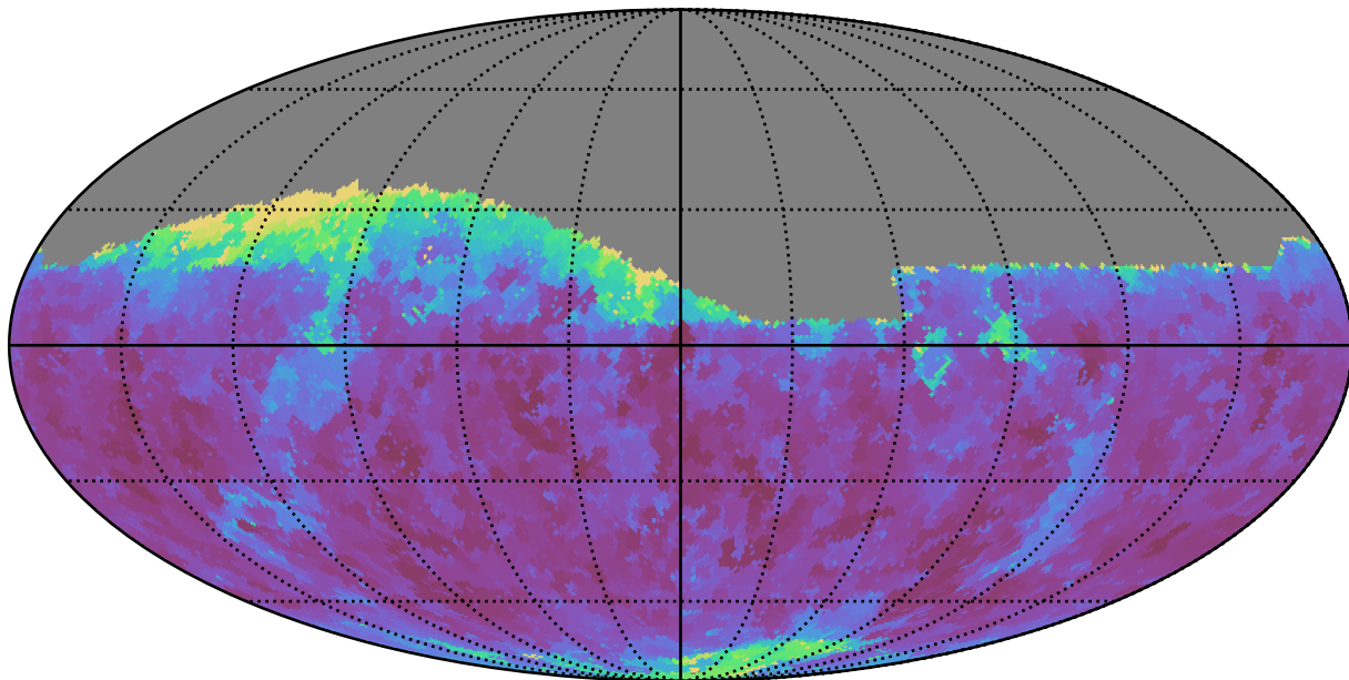
ddf_acor_sf10_lsf20_lsr20_v3.4_10yrs Yr 1 i band: Min seeingEff
