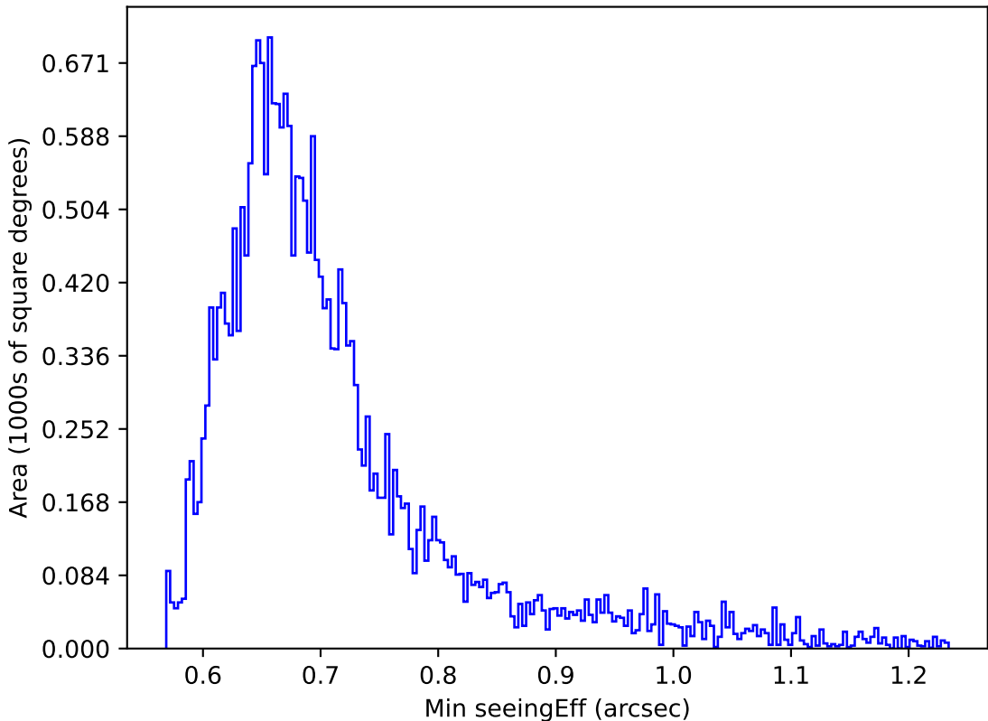
ddf_acor_sf10_lsf20_lsr20_v3.4_10yrs Yr 1 i band: Min seeingEff
