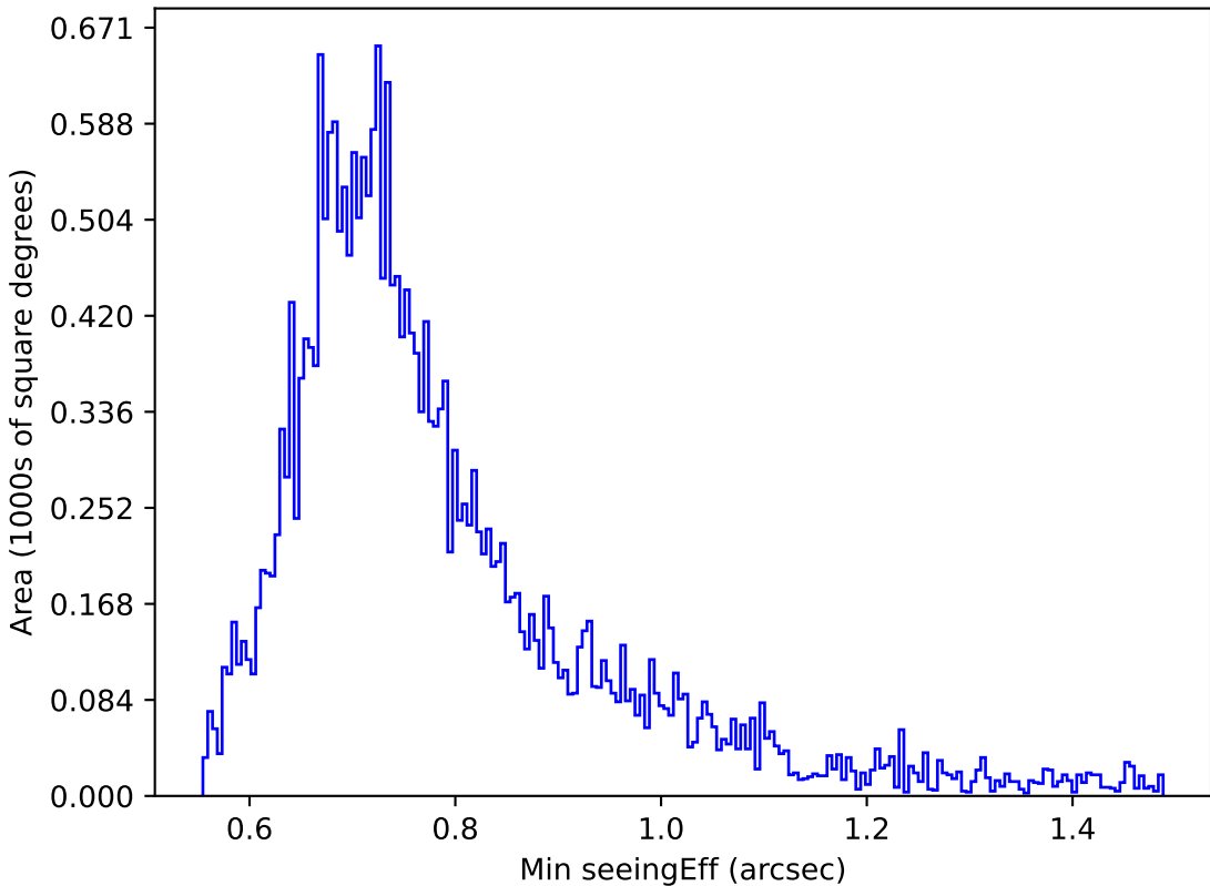
ddf_acor_sf10_lsf20_lsr20_v3.4_10yrs Yr 1 g band: Min seeingEff
