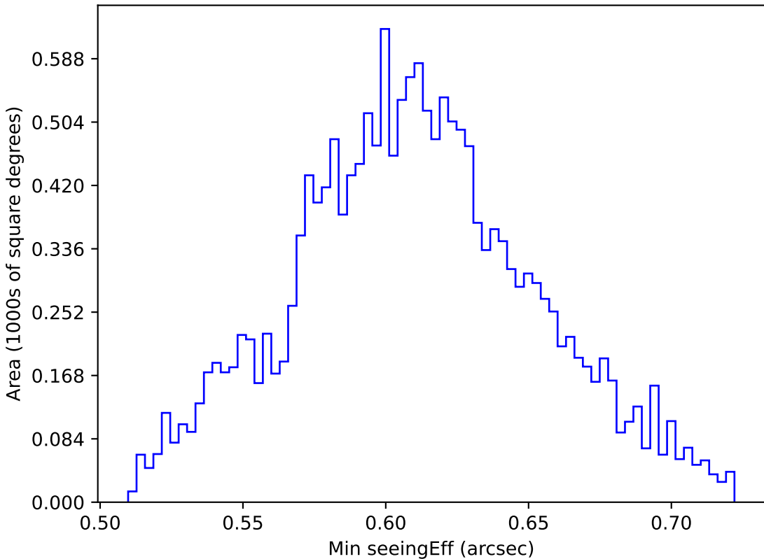
ddf_acor_sf10_lsf20_lsr20_v3.4_10yrs WFD z band: Min seeingEff
