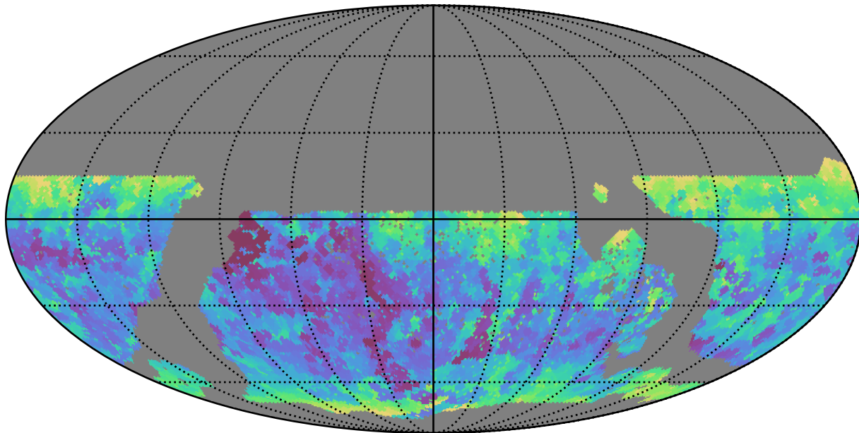
ddf_acor_sf10_lsf20_lsr20_v3.4_10yrs WFD y band: Min seeingEff
