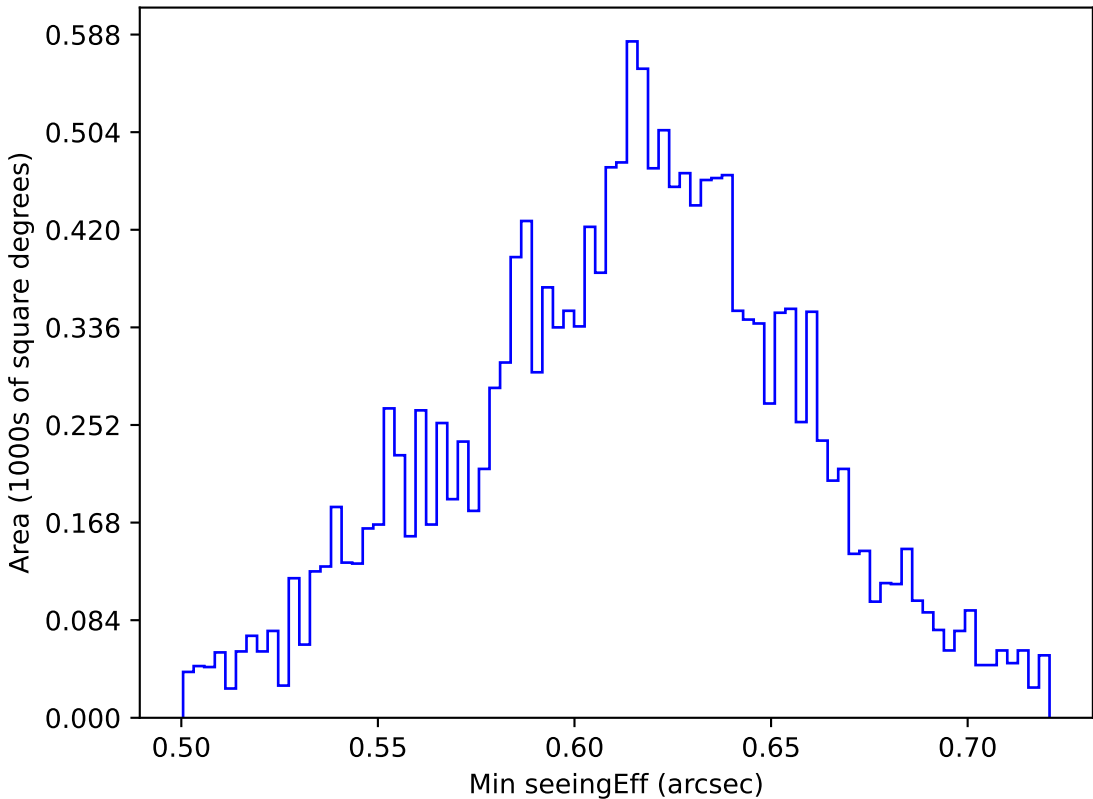
ddf_acor_sf10_lsf20_lsr20_v3.4_10yrs WFD r band: Min seeingEff
