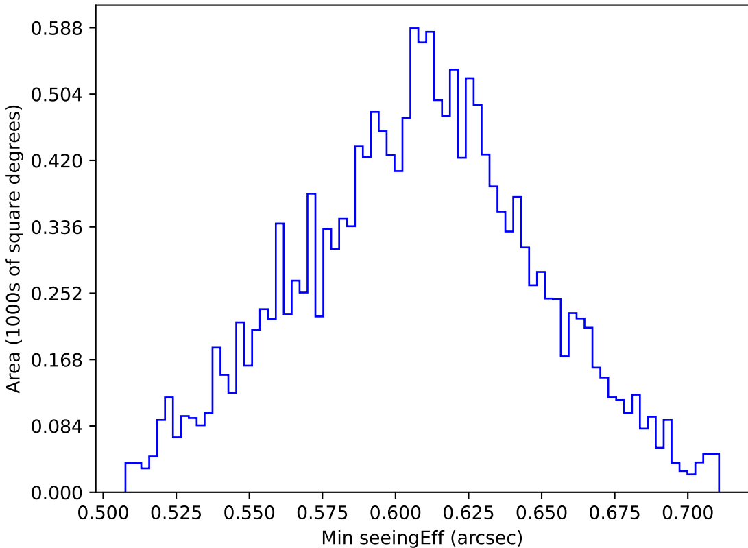
ddf_acor_sf10_lsf20_lsr20_v3.4_10yrs WFD i band: Min seeingEff
