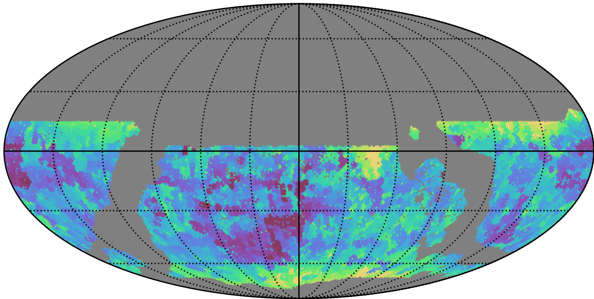
ddf_acor_sf10_lsf20_lsr20_v3.4_10yrs WFD g band: Min seeingEff
