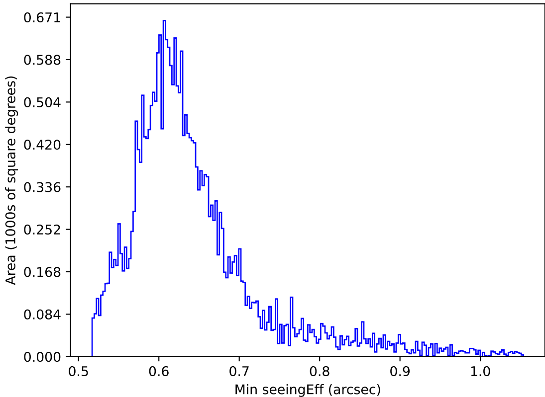
ddf_acor_sf10_lsf20_lsr20_v3.4_10yrs All sky z band: Min seeingEff
