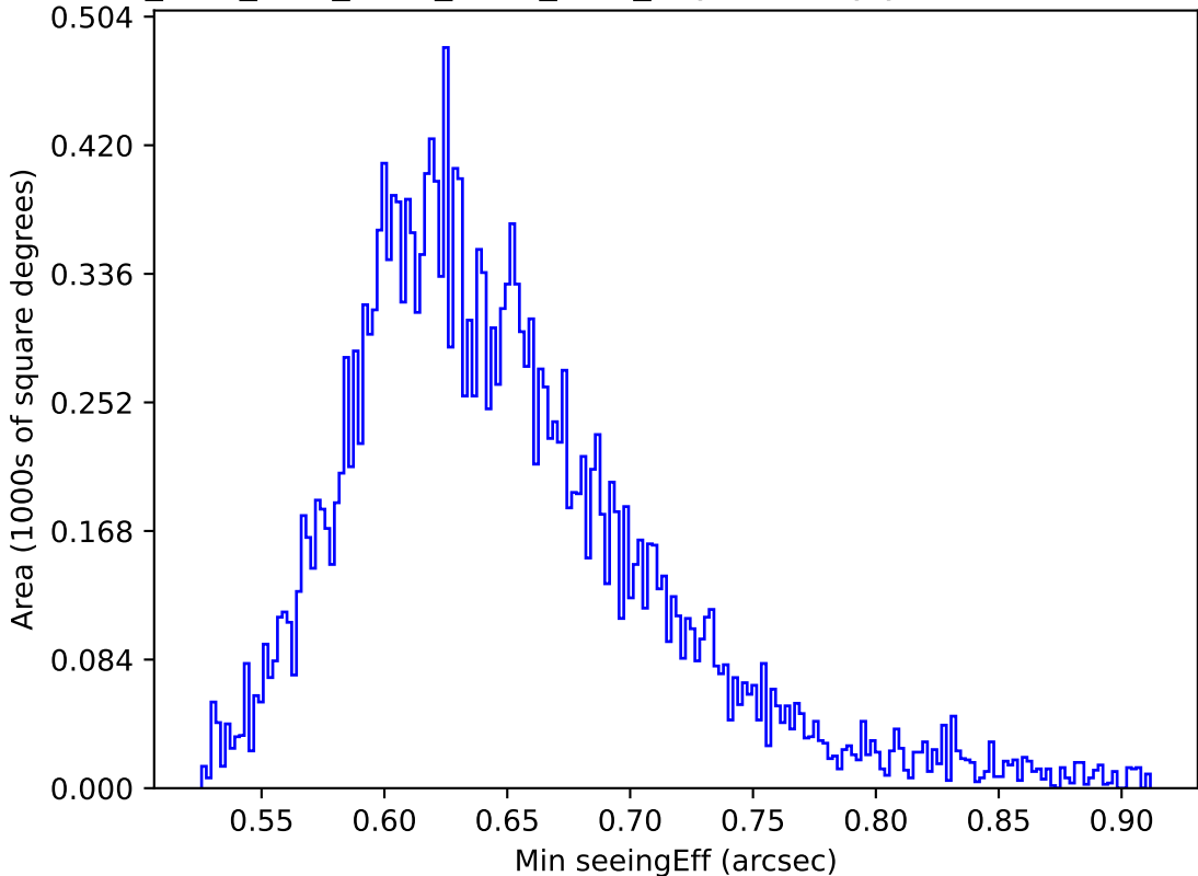
ddf_acor_sf10_lsf20_lsr20_v3.4_10yrs All sky y band: Min seeingEff
