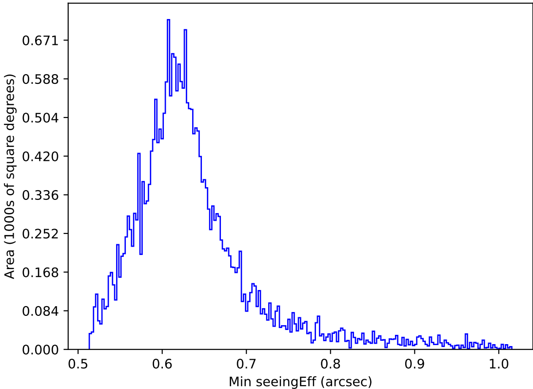
ddf_acor_sf10_lsf20_lsr20_v3.4_10yrs All sky i band: Min seeingEff
