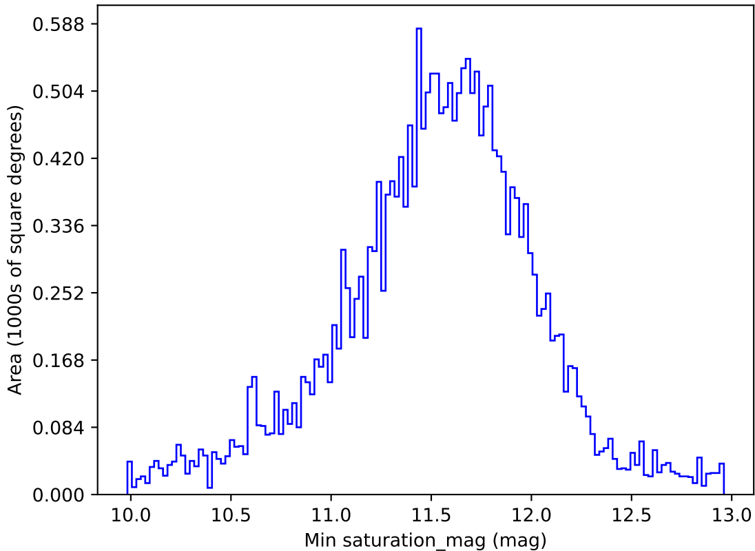
ddf_acor_sf10_lsf20_lsr20_v3.4_10yrs All sky u band: Min saturation_mag
