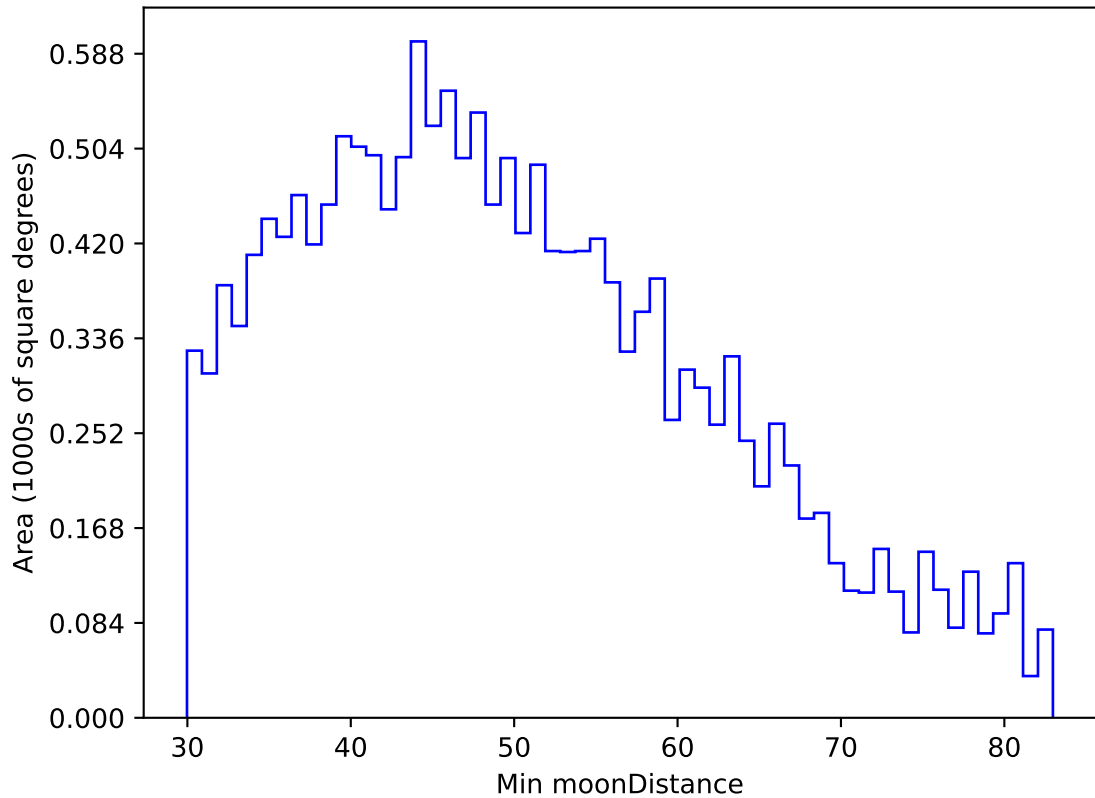
ddf_acor_sf10_lsf20_lsr20_v3.4_10yrs WFD u band: Min moonDistance
