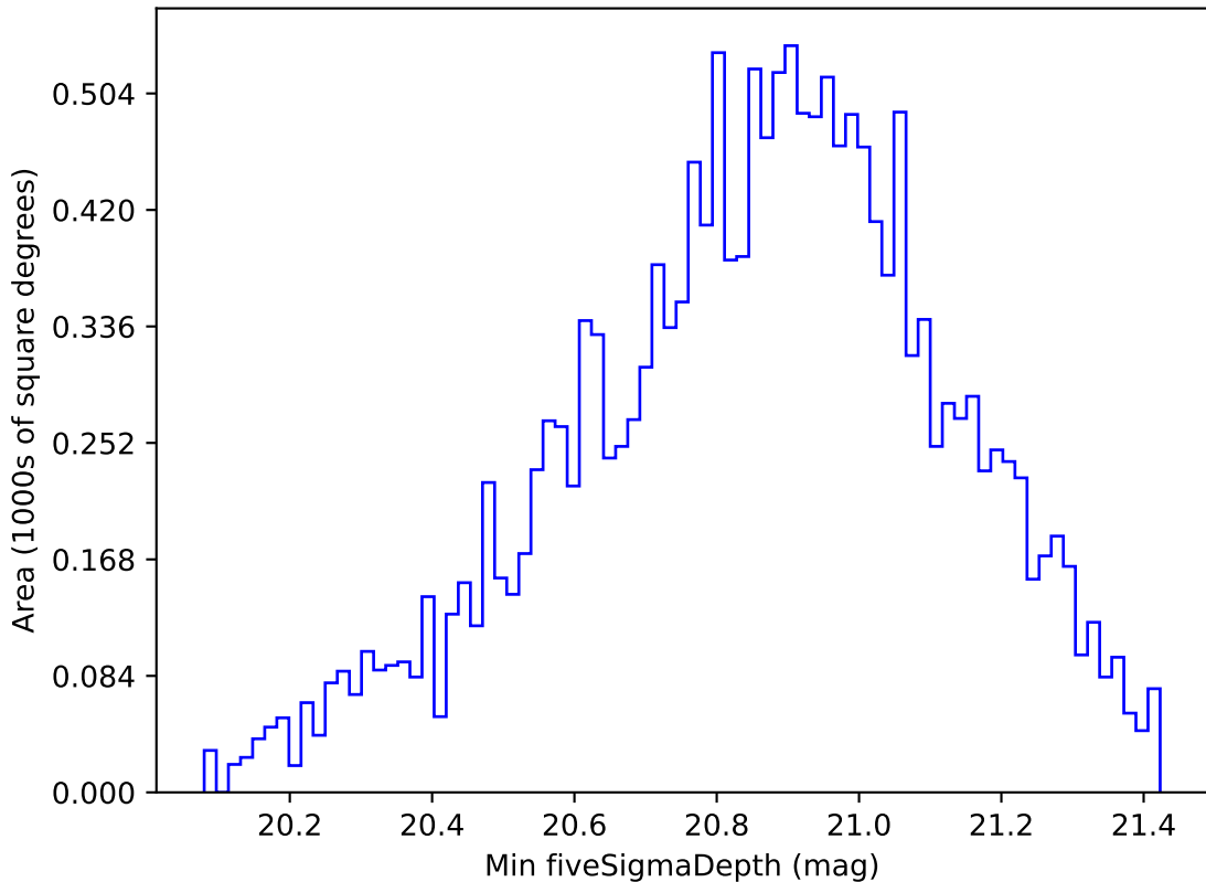
ddf_acor_sf10_lsf20_lsr20_v3.4_10yrs WFD y band: Min fiveSigmaDepth
