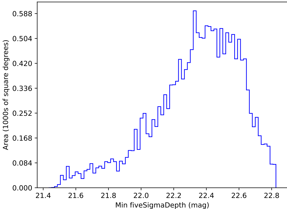
ddf_acor_sf10_lsf20_lsr20_v3.4_10yrs WFD u band: Min fiveSigmaDepth
