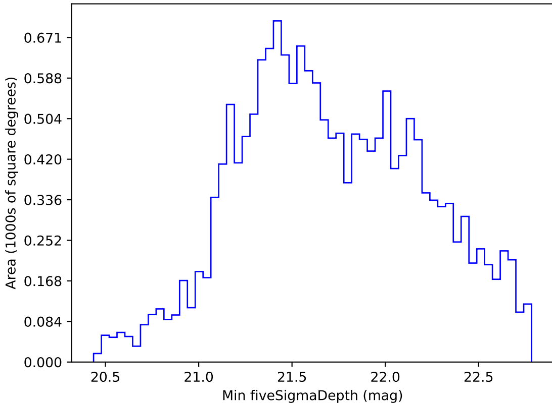
ddf_acor_sf10_lsf20_lsr20_v3.4_10yrs WFD i band: Min fiveSigmaDepth
