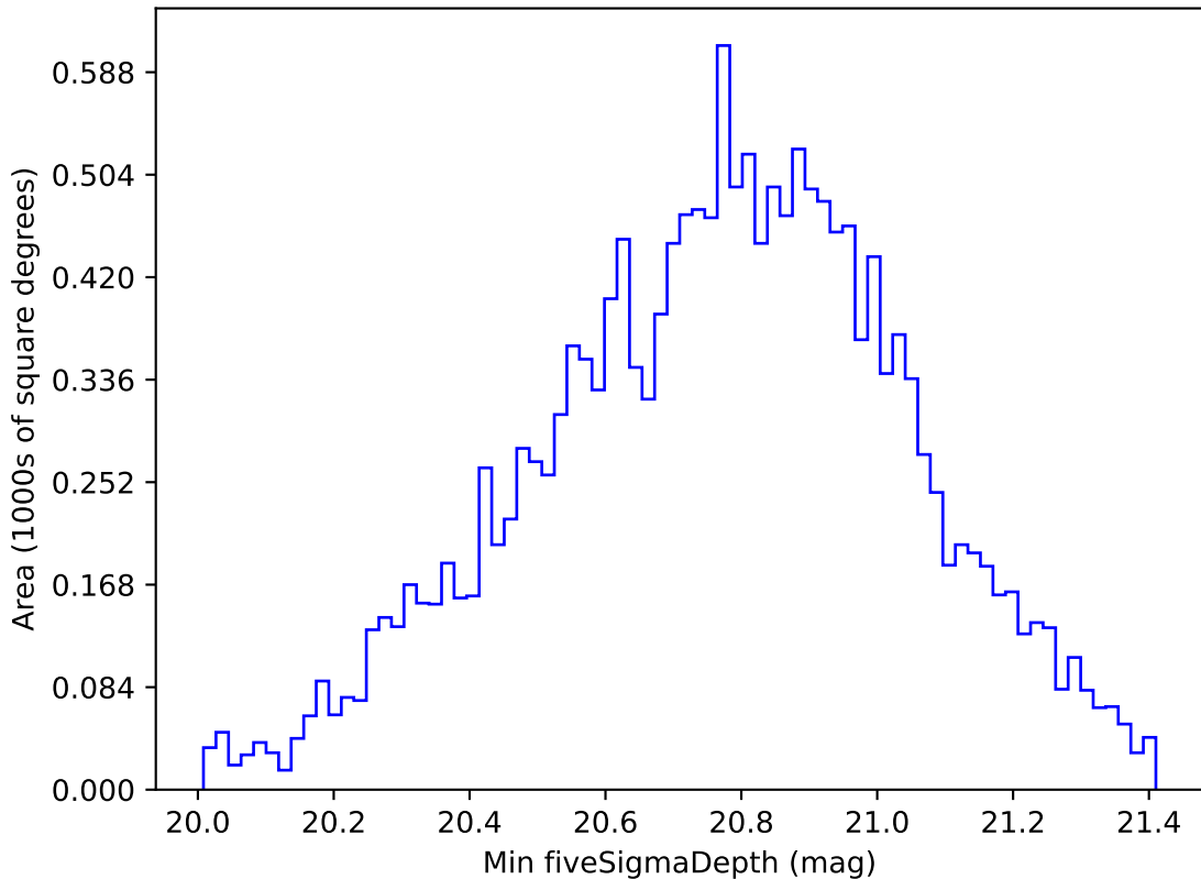
ddf_acor_sf10_lsf20_lsr20_v3.4_10yrs WFD all bands: Min fiveSigmaDepth
