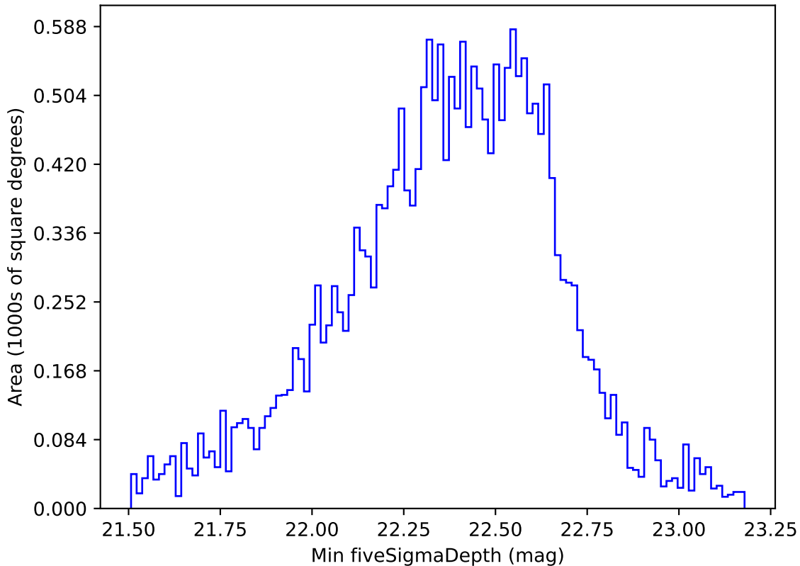
ddf_acor_sf10_lsf20_lsr20_v3.4_10yrs All sky u band: Min fiveSigmaDepth
