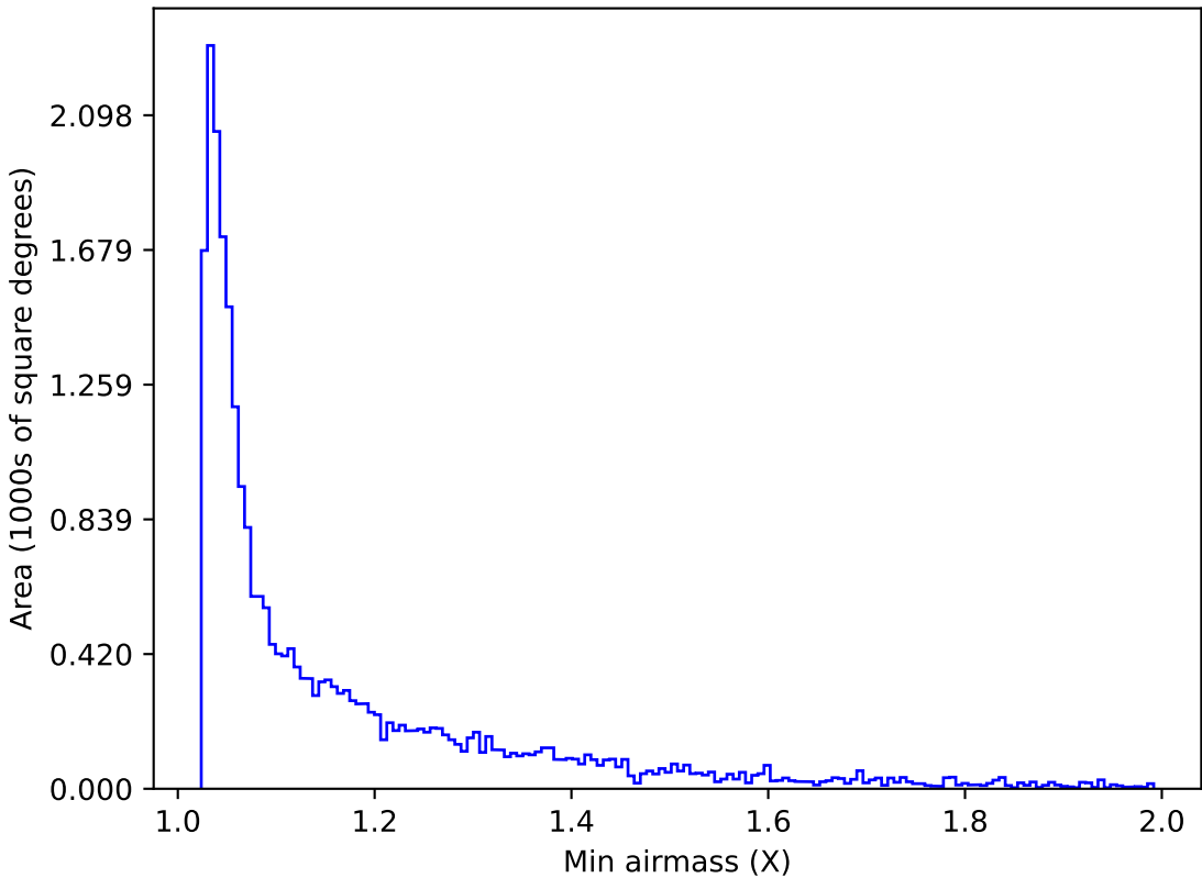
ddf_acor_sf10_lsf20_lsr20_v3.4_10yrs Yr 1 z band: Min airmass
