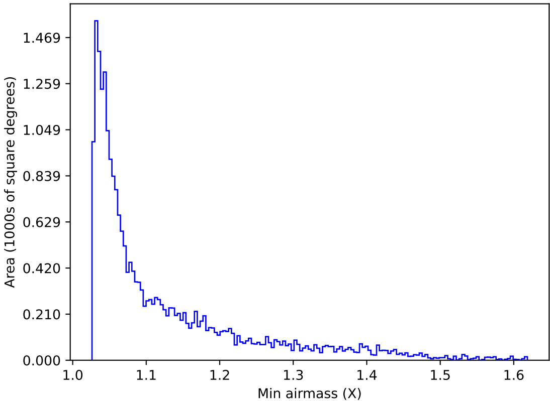
ddf_acor_sf10_lsf20_lsr20_v3.4_10yrs Yr 1 y band: Min airmass
