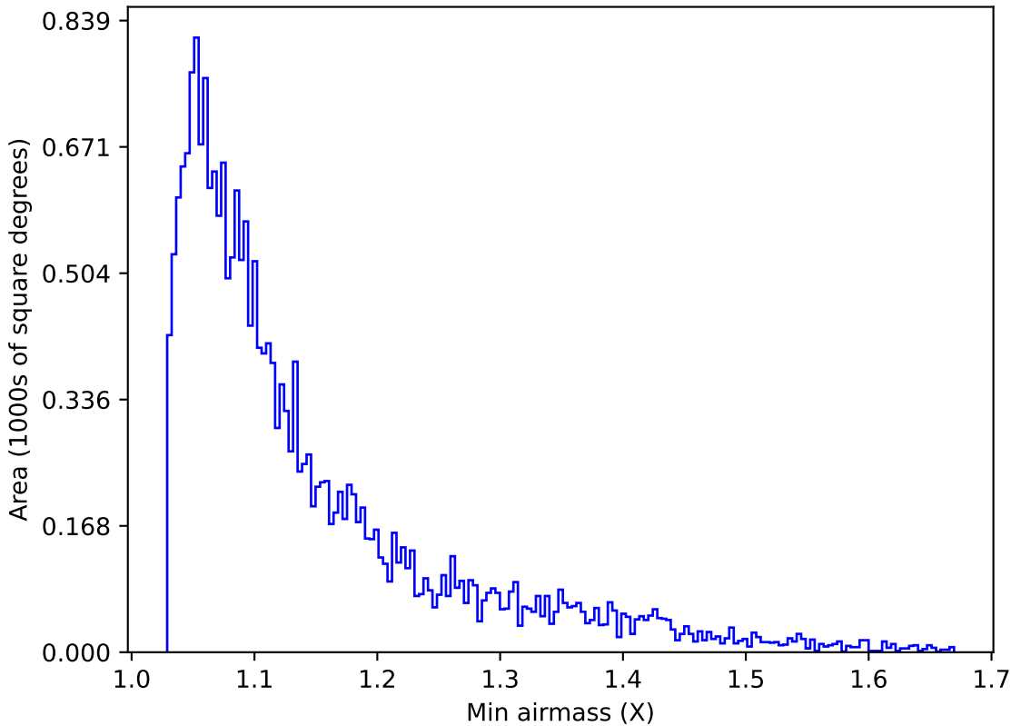
ddf_acor_sf10_lsf20_lsr20_v3.4_10yrs Yr 1 u band: Min airmass
