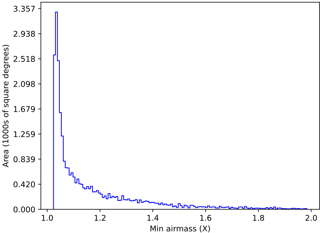
ddf_acor_sf10_lsf20_lsr20_v3.4_10yrs Yr 1 i band: Min airmass
